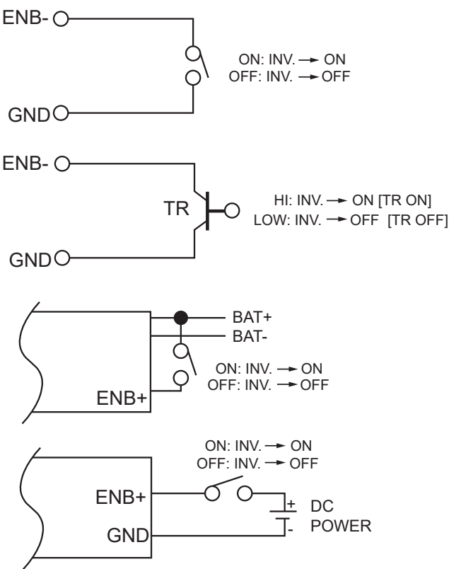
Dry contact terminal definition
