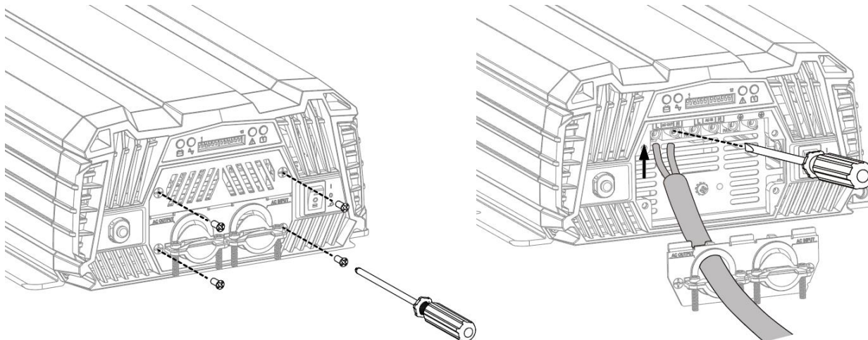
Fig. 9 : SC-1200 / 2000 Installation
