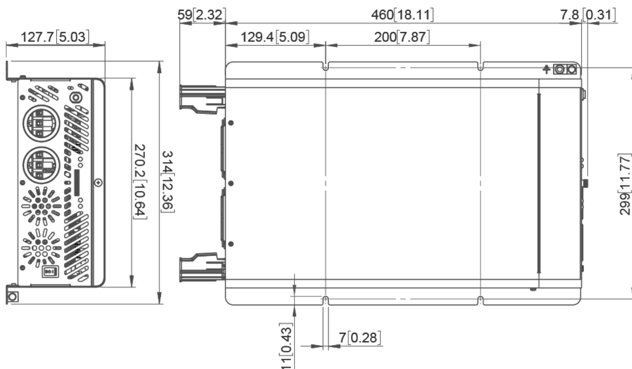
Fig. 4 : SC 3000 Mechanical drawings
