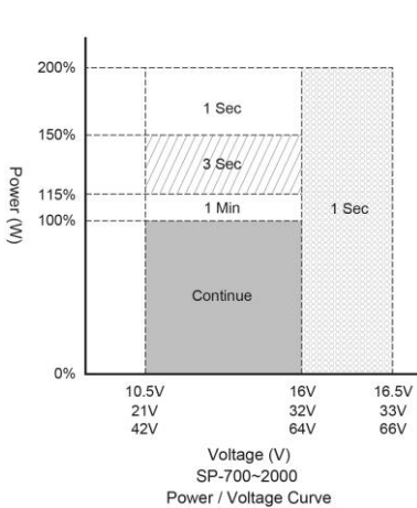
Figure 1. SP-700~2000 Output power vs. input voltage
